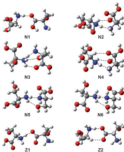
Figure 3. Lowest-energy isomers of [\text{H}(\text{Ser})_2]^+ optimized by B3LYP/6-311++G(d,p), with six neutral ( N1–N6 ) and two zwitterionic ( Z1–Z2 ) structures. The red, blue, gray, and white spheres denote O, N, C, and H atoms, respectively. Note that the structures of N2–N6 are all dominated by linear neutral and ionic \text{N–H}^+\cdots\text{N} hydrogen bonds, instead of \text{N–H}^+\cdots\text{O} , because the amino group has a much higher proton affinity than both the carboxy group on the C terminus and the hydroxy group on the serine side chain.
